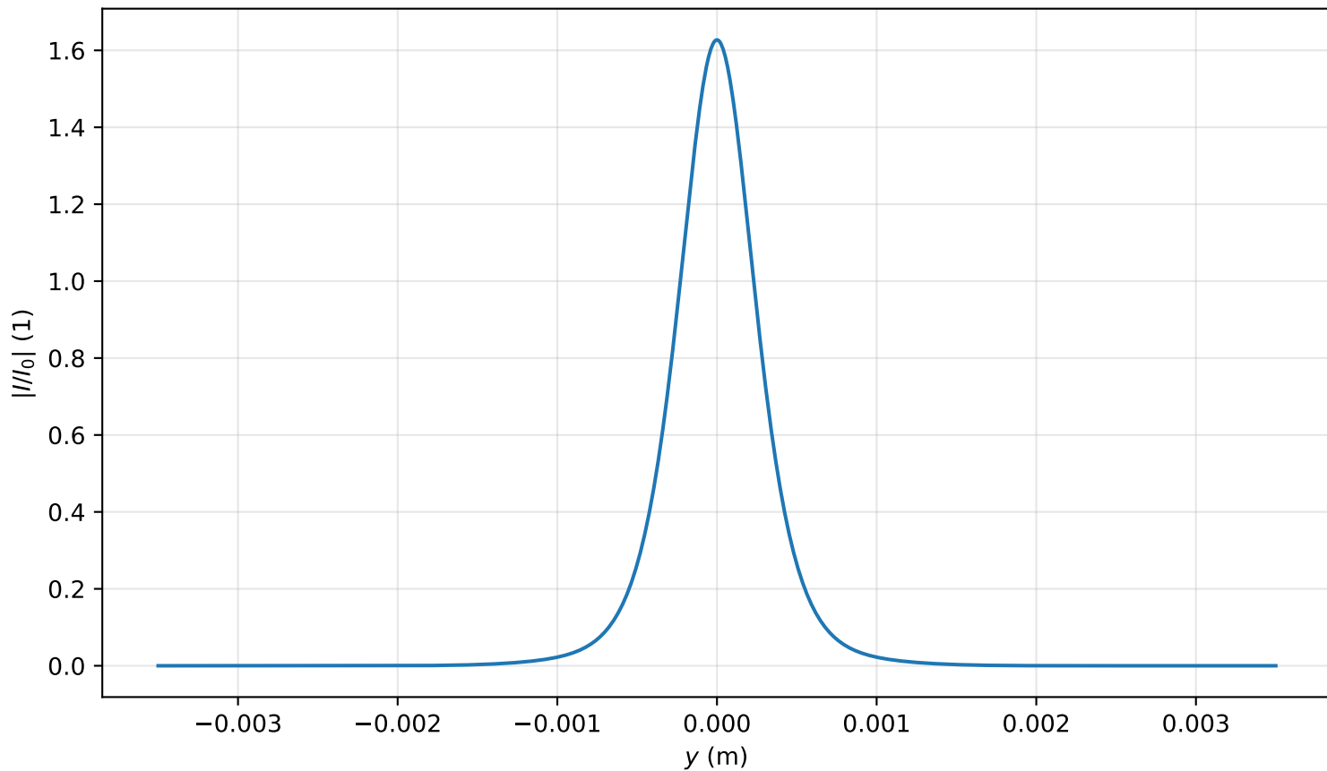
Intensity profile I(x=0, y, z=1.911)/I_0 , P_{in}=0.9P_{cr} , artificial time
